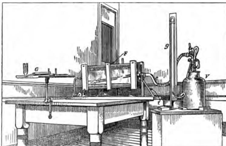
FIG. 57a.—Disposition of coronal apparatus for measuring atmospheric nucleation ("dust"). V , vacuum chamber; F , fog chamber; G , goniometer; g , gage; e , exhaust pipe; t , support for trunnions. Influx pipe at left end of fog chamber.
